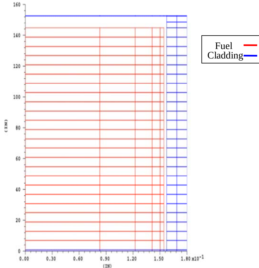
Typical PWR Model
