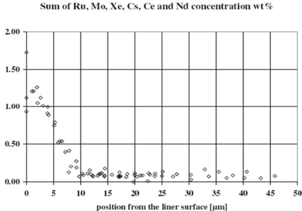
Figure 5 Sum of selected fission products measured by EPMA at the inner surface of the liner
