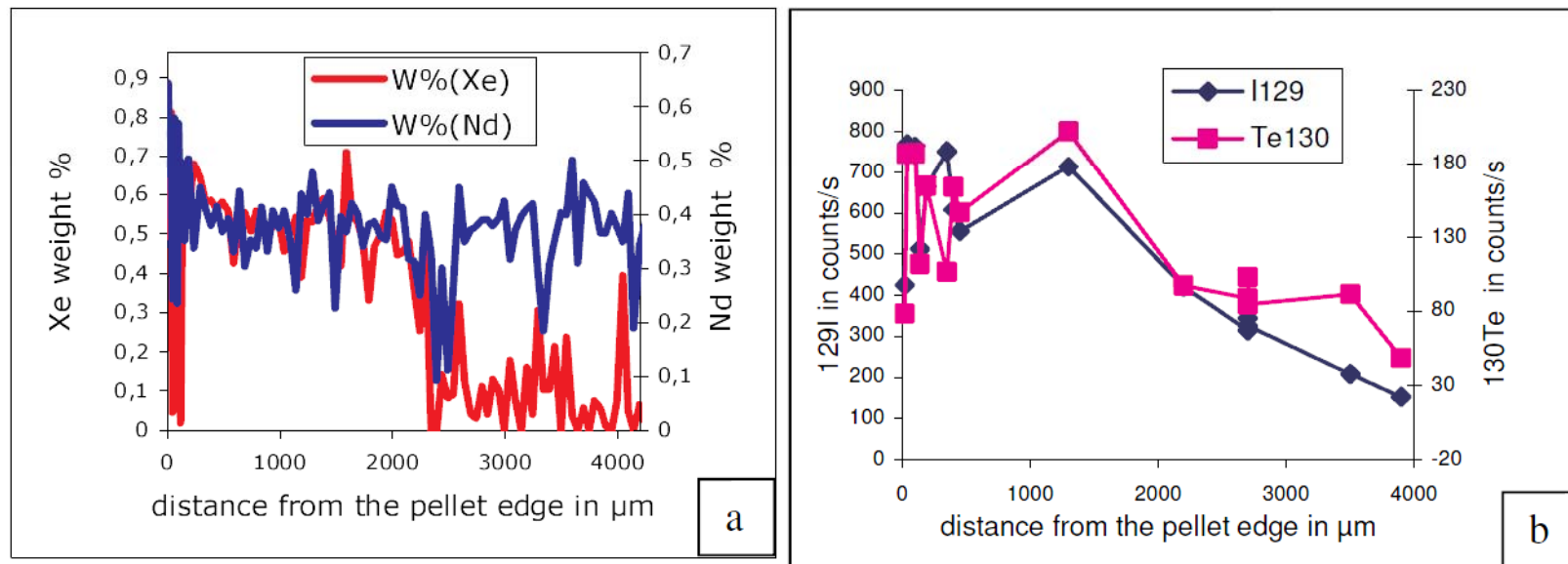
Figure 4 : EPMA quantitative concentration profile of xenon and neodymium (a) and SIMS profile of iodine and tellurium measured along the purple radius shown on figure 3.
