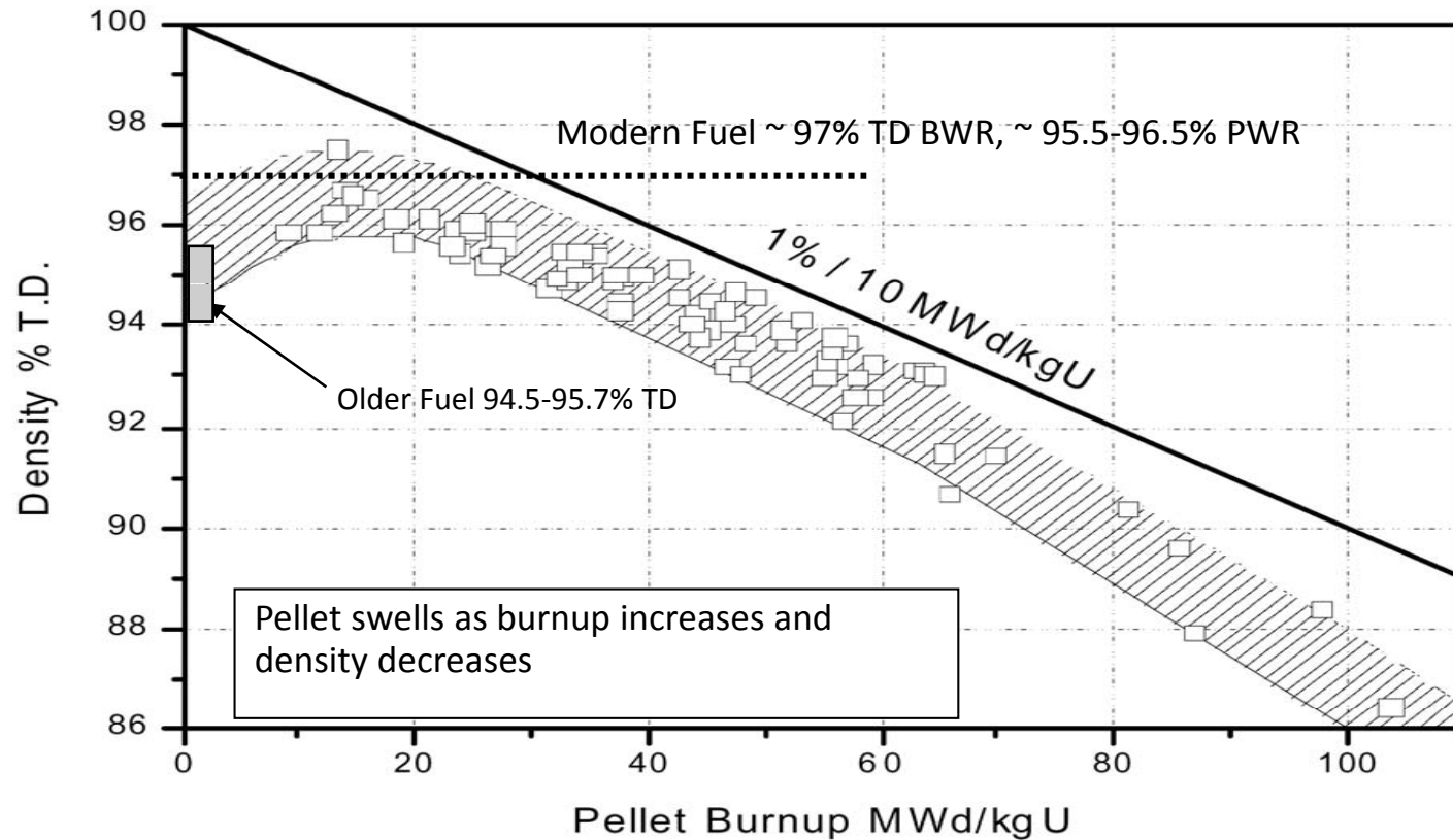
Fuel Pellet Density Trend with Pellet Exposure (Matrix Swelling Rate Shown for Comparison)
