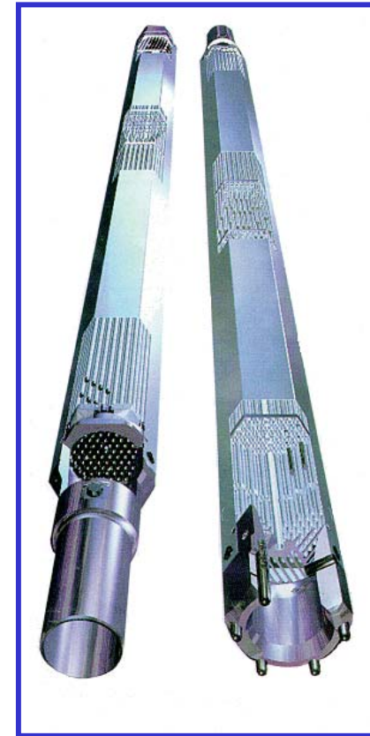
fuel assembly
