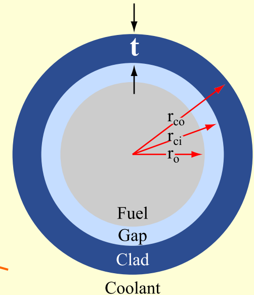
Cross Section of a Representative Fuel Pin (not drawn to scale)
