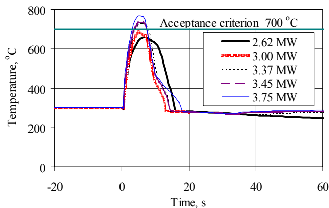
Fig. 4. Peak fuel cladding temperature in the FC connected to GDH with fail to close check valve
