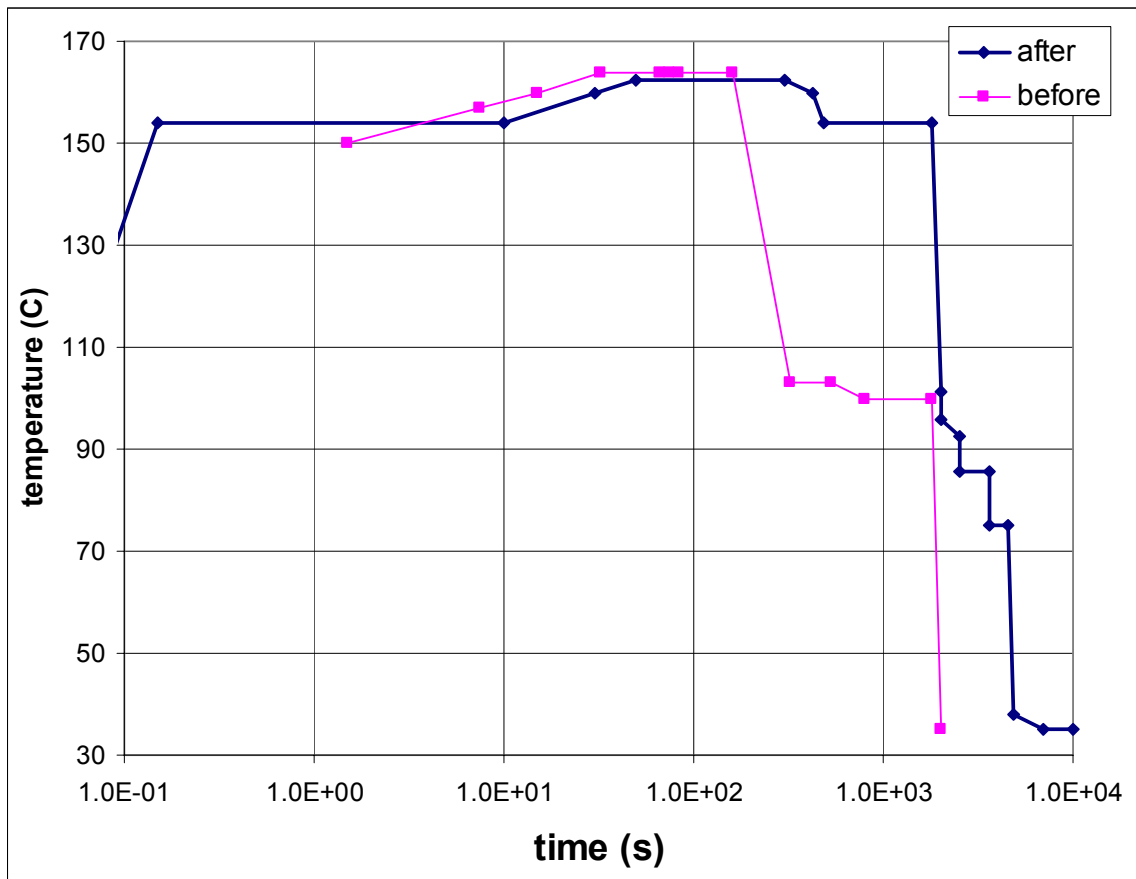
Figure 6 MSLB, MFLB and AFWPTB limiting temperature profiles for IB
