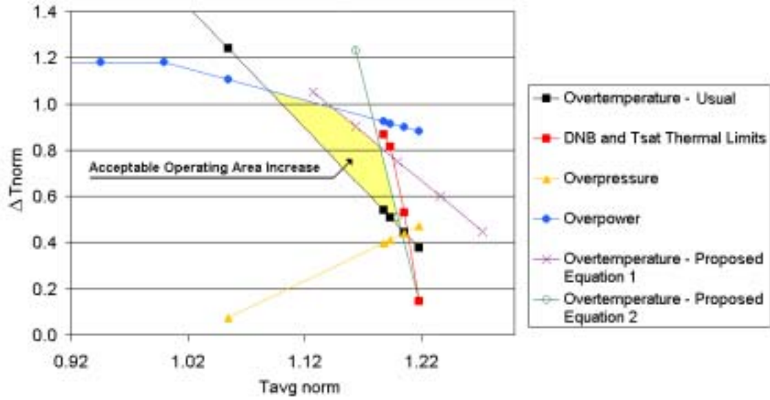
Figure 11 - Normalized Protection Curves and DNB and T_{sat} Limits – Pressure 14 MPa
