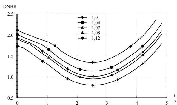
Figure 6 - Influence of K_{eng}
