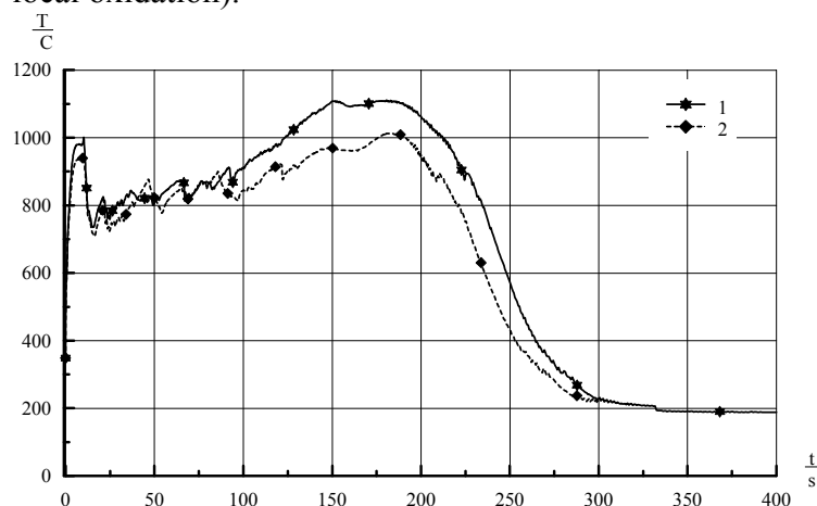
Figure 9 - Influence of gas gap conductance 1 – conductance according to design approach 2 – conductance for probability 95 %
