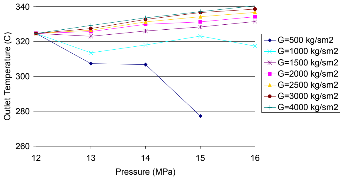
Figure 2 – Outlet Temperature versus pressure.
