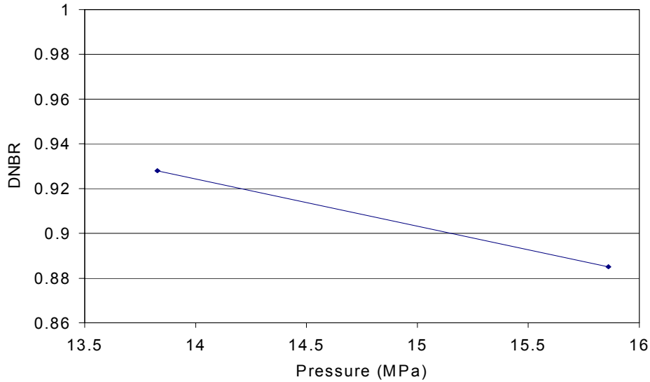
Figure 9 – DNBR (EPRI) versus pressure for Constant T_{in} and G \cong 720 \text{ kg s}^{-1}\text{m}^2 .
