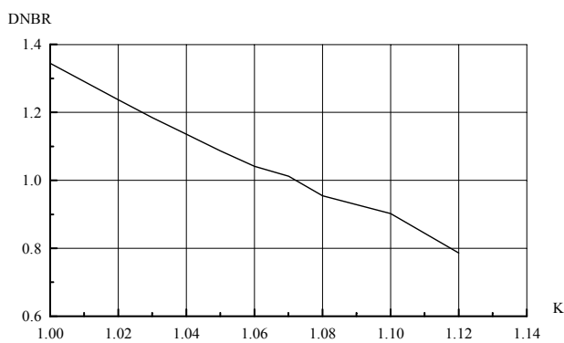
Figure 7 - Minimum DNBR versus K_{eng}
