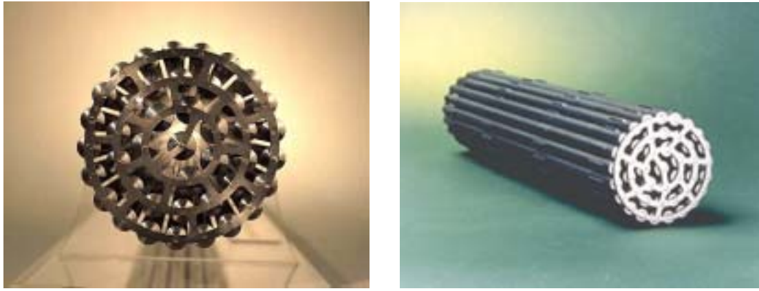
Fig. 3. CANFLEX fuel
