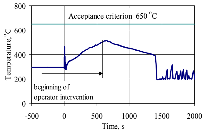
Fig. 3. Peak temperature of fuel channel wall in maximum loaded FC connected to GDH with fail to close check valve
