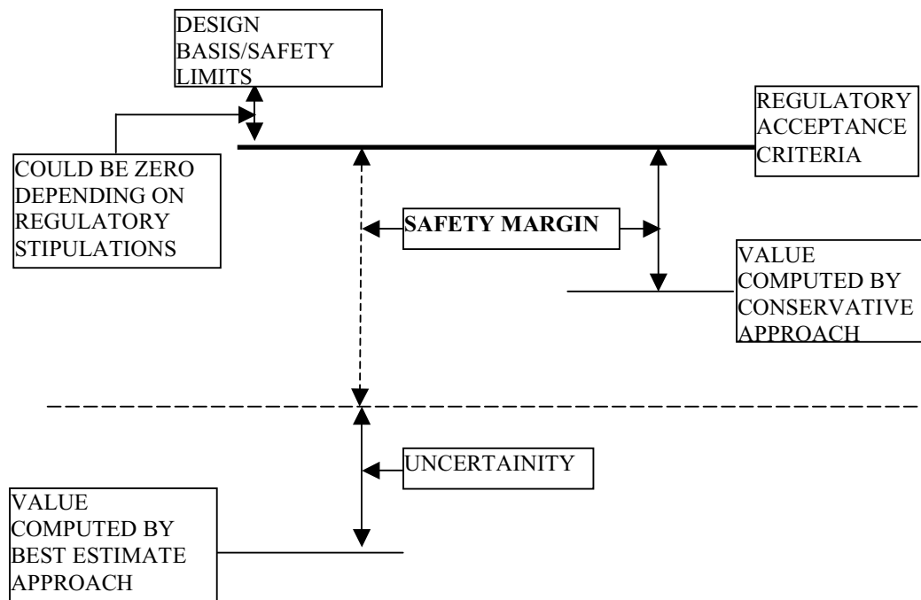
Fig. 1 Safety Margins for Deterministic (Accident) Analysis
