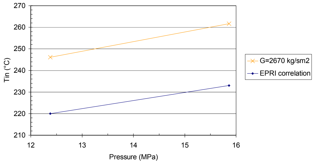
Figure 6 – Inlet temperature versus pressure, DNBR=1 and G \cong 2,670 \text{ kg s}^{-1}\text{m}^2 .
