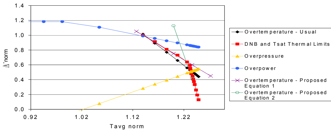
Figure 10-Normalized Protection Curves and DNB and T_{sat} Limits– Pressure 15.5 MPa
