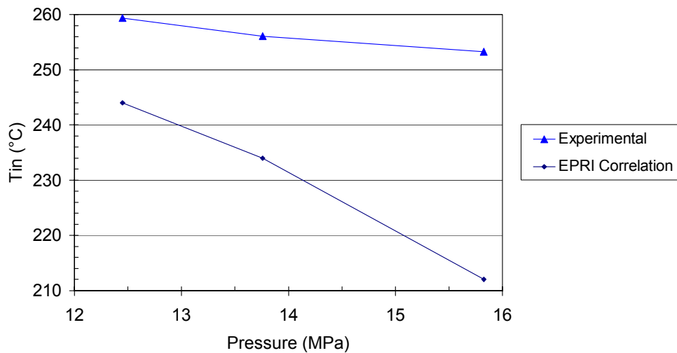
Figure 4 – Inlet temperature versus pressure for DNBR=1 and G \cong 1,370 \text{ kg s}^{-1}\text{m}^2 .
