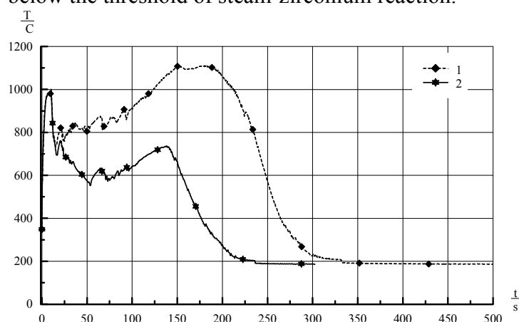
Figure 10 – Influence of residual heat 1 – for interval 3\sigma 2 - for probability 95 %
