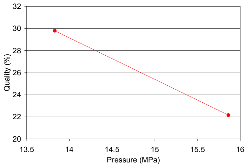
Figure 7 – Critical quality versus pressure for Constant T_{in} and G \cong 720 \text{ kg s}^{-1}\text{m}^2 .
