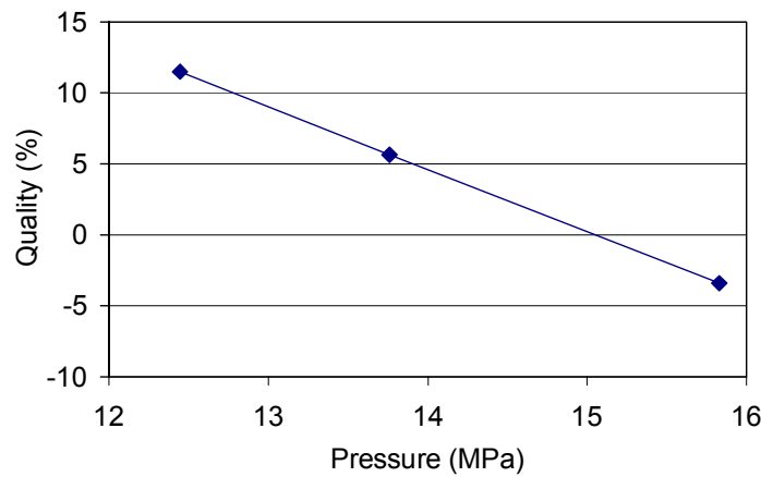
Figure 3 – Critical quality versus pressure for constant heat flux and G \cong 1,370 \text{ kg s}^{-1}\text{m}^2 .
