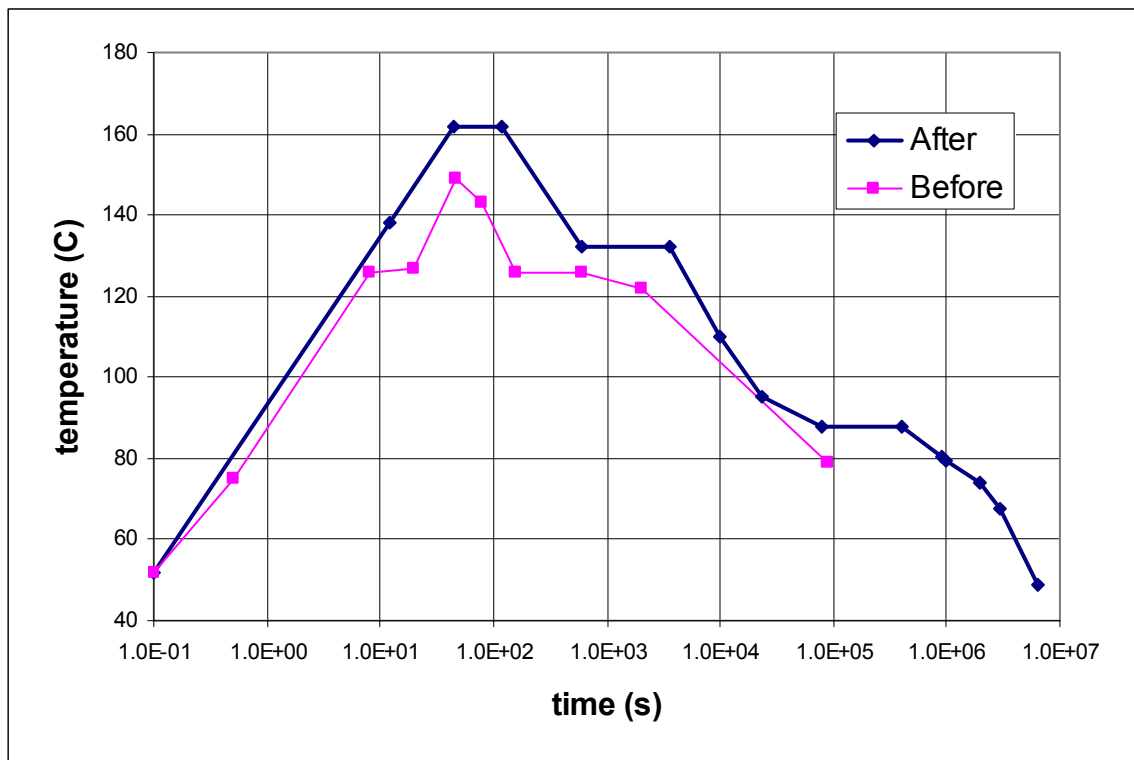
Figure 2 Containment Temperature Envelope
