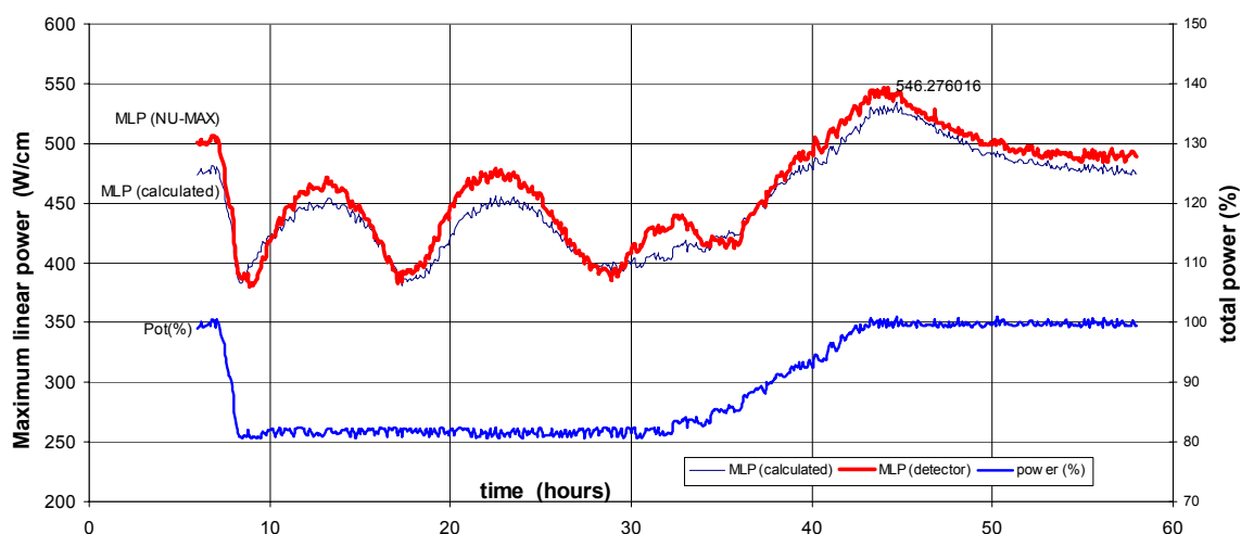
Figure 2 Maximum Linear Power
