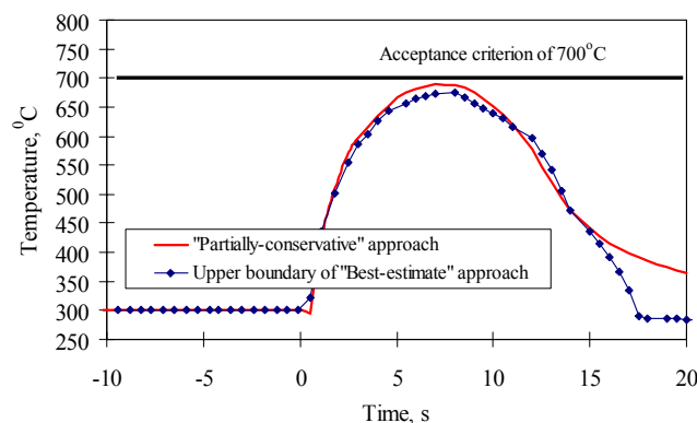
Fig. 7. Comparison of the peak fuel cladding temperature in the fuel channel of 2.62 MW, connected to GDH with failure to close check valve in case of “partially-conservative” calculation and “best-estimate” calculation with uncertainty and sensitivity analysis
