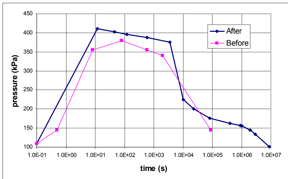
Figure 1 Containment Pressure Envelope
