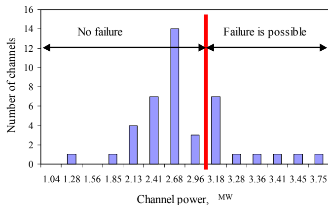
Fig. 8. Real distribution of FC power in the most loaded GDH at 4200 MW power level
