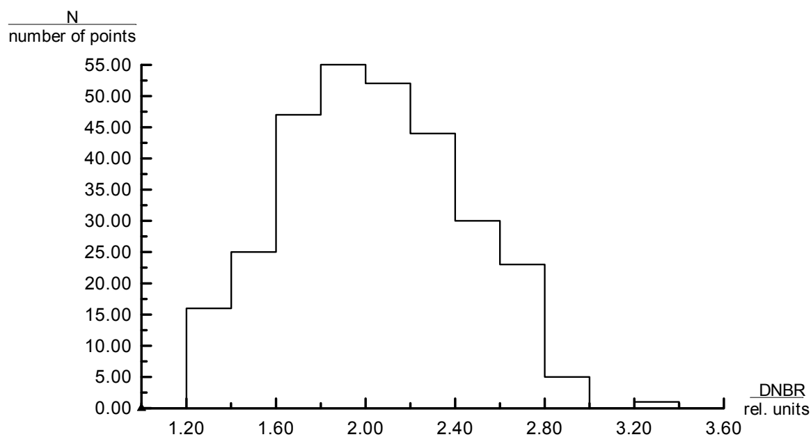
Figure 11 – Histogram of distribution of minimum DNBR
