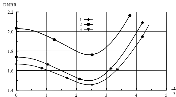
Figure 2 – Influence of power shapes during de-energization of all RCPs
