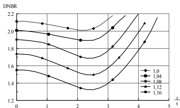
Figure 4 - Influence of K_{eng}
