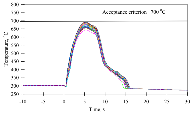
Fig. 5. Fuel cladding temperatures at the location of 2.75 m from the core bottom obtained using SUSA generated runs from RELAP5 calculations
