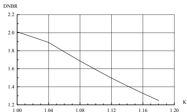
Figure 5 - Minimum DNBR versus K_{eng}
