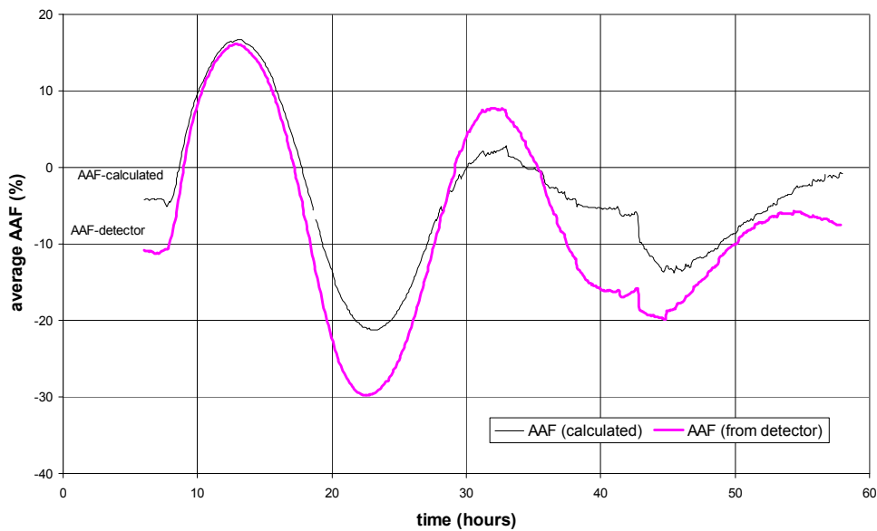
Figure 3 Axial Asymmetric Factor
