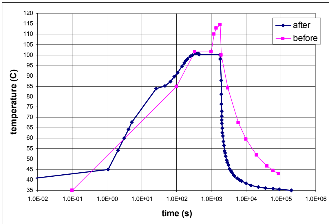
Figure 7 Typical CVCS Line Break temperature profile in room AB room with potential break location
