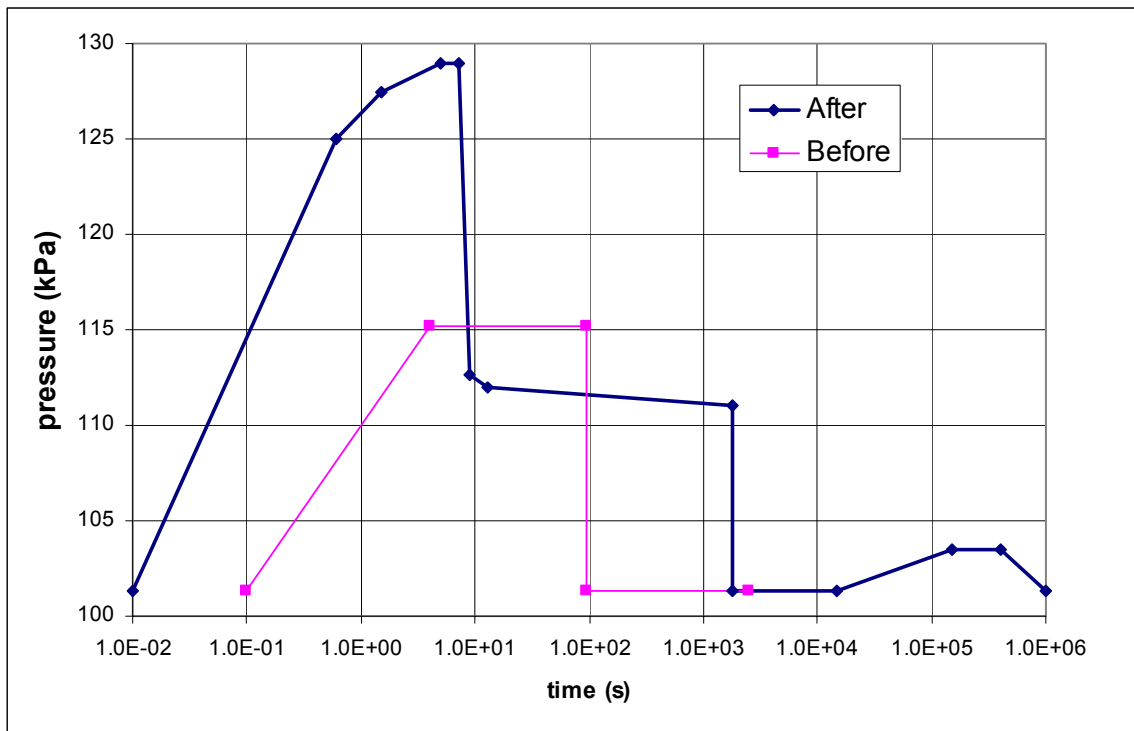
Figure 4 Pressure for Steam Generator Blowdown Break (SGBDB) in IB rooms with potential break locations
