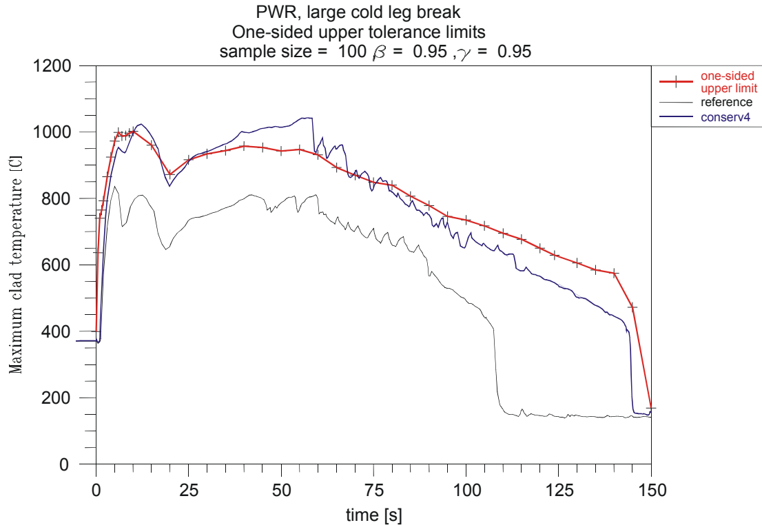
Figure 1: Calculated one-sided uncertainty limit and best estimate reference calculation compared with a “conservative” calculation of rod clad temperature for a reference reactor during a postulated double ended offset shear cold leg break.
