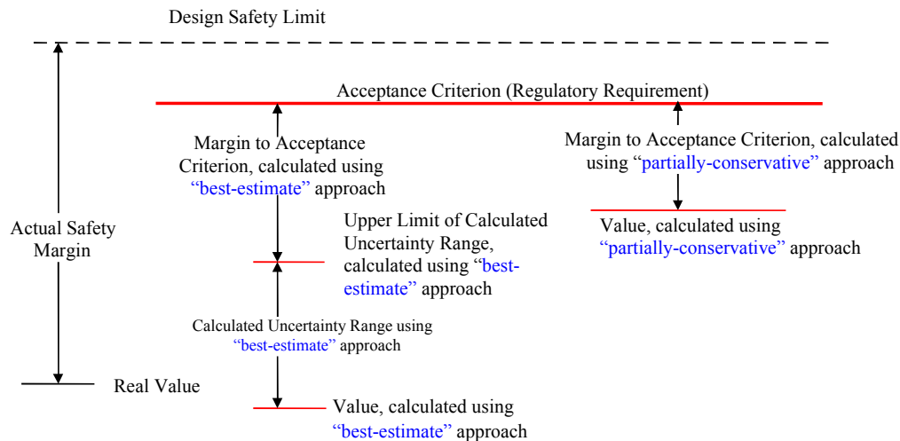
Fig. 6. Illustration of the margin to the acceptance criterion
