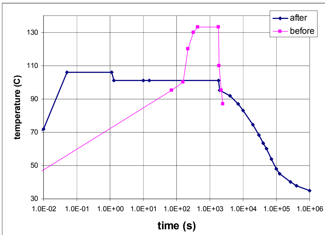
Figure 3 Temperature for Steam Generator Blowdown Break (SGBDB) in IB rooms with potential break locations
