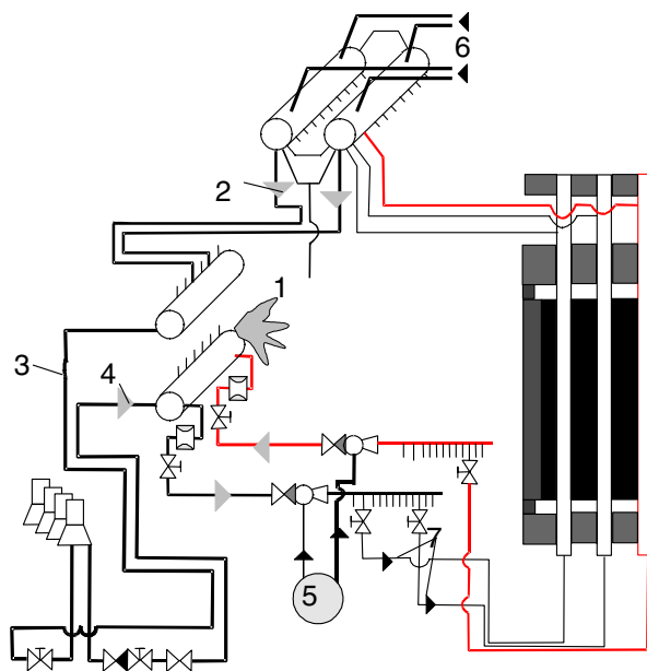
Fig. 1. MCP pressure header break with failure to close check valve of one GDH. Structure of coolant flows: 1 – break of PH; 2 – overflow of coolant from DS; 3 – MCP suction piping; 4 – coolant discharge from MCP pressure piping; 5 – ECCS water supply; 6 – steam supply from intact loop of the MCC; 7 – coolant supply into reactor core
