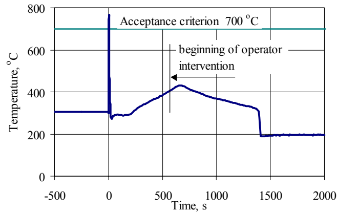
Fig. 2. Peak temperature of fuel cladding in maximum loaded FC connected to GDH with fail to close check valve
