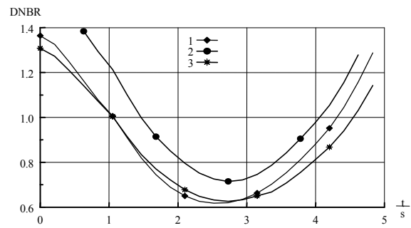
Figure 3 - Influence of power shapes during seizure of one RCP
