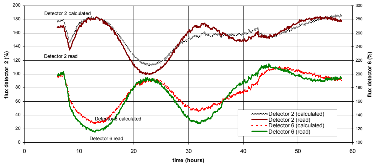
Figure 4 Thermal Flux on In-Core Detectors
