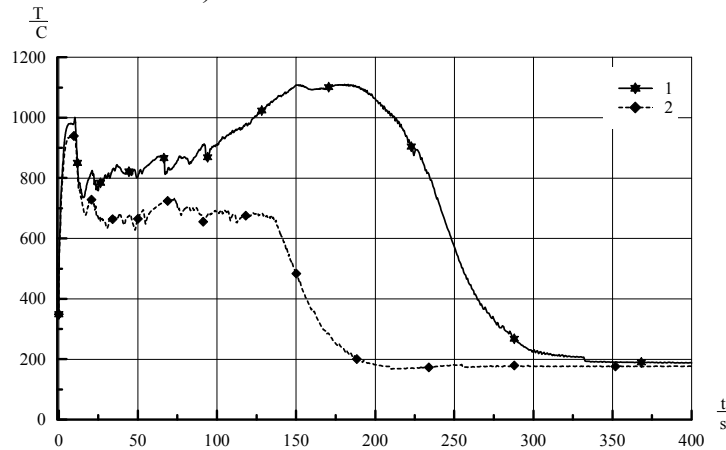
Figure 8 - Influence of linear heat rate
