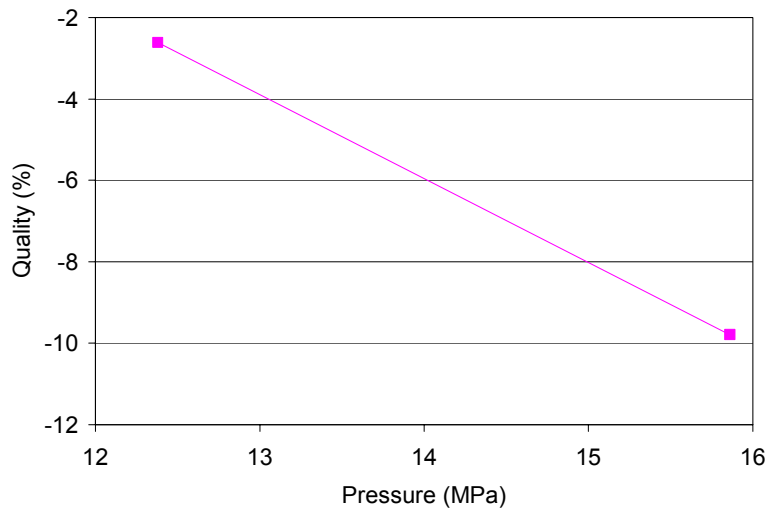
Figure 5 – Critical quality versus pressure – G \cong 2,670 \text{ kg s}^{-1}\text{m}^2 .
