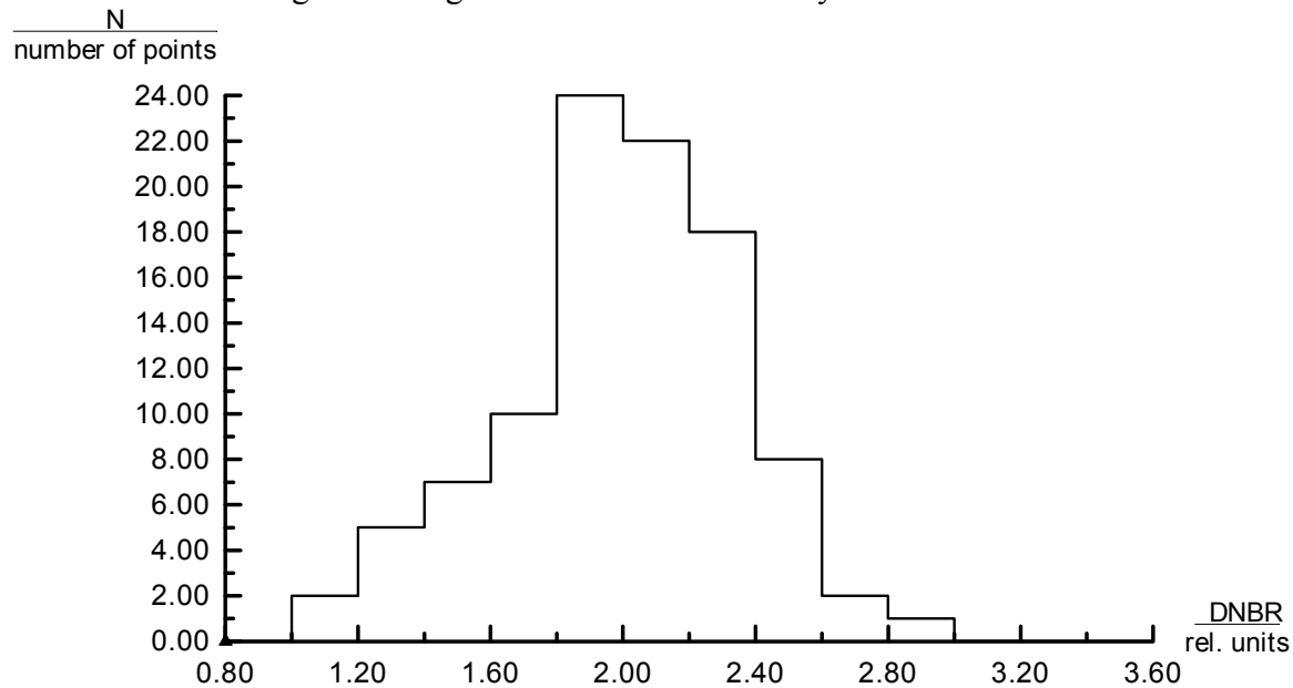
Figure 12 - Histogram of distribution of minimum DNBR
