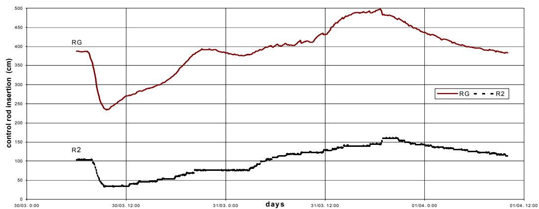
Figure 1 Control Rod Positions in a typical load cycle
