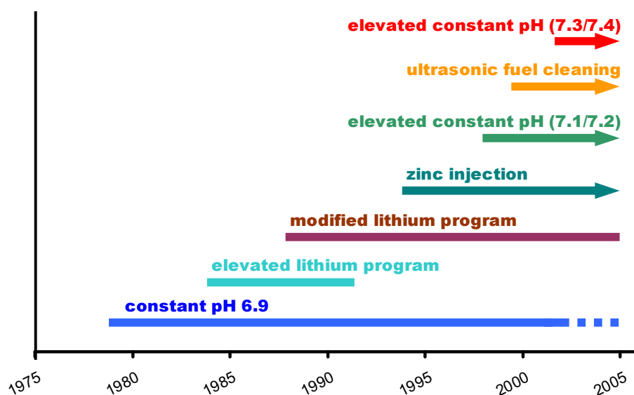
Figure 3. Evolution of recommended PWR water chemistry
