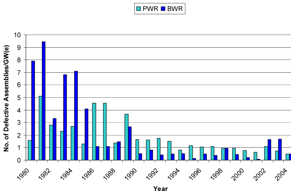
Figure 5. Fuel failure rates in US plants.
