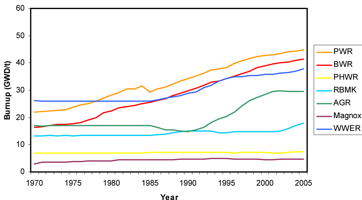
Figure 2. Trends in fuel burnup for different types of reactors
