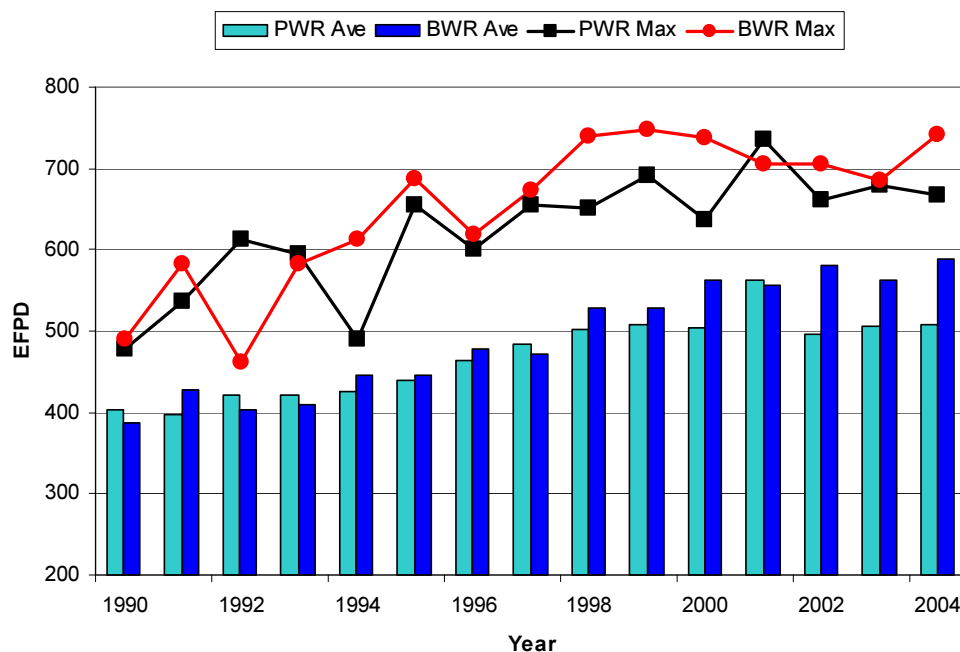
Figure 1. Increasing average cycle lengths for fuel elements in PWRs and BWRs in the USA.
