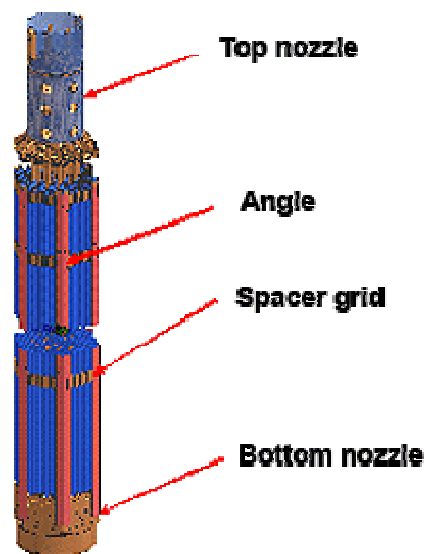
Figure 4. Angle stiffening on the advanced TVSA fuel assembly for a WWER 1000 reactor
