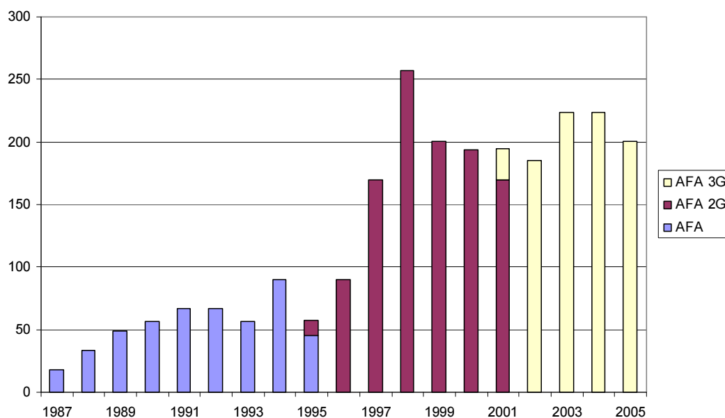
Figure 6. Number and type of MOX fuel assemblies loaded in French 900MW PWRs
